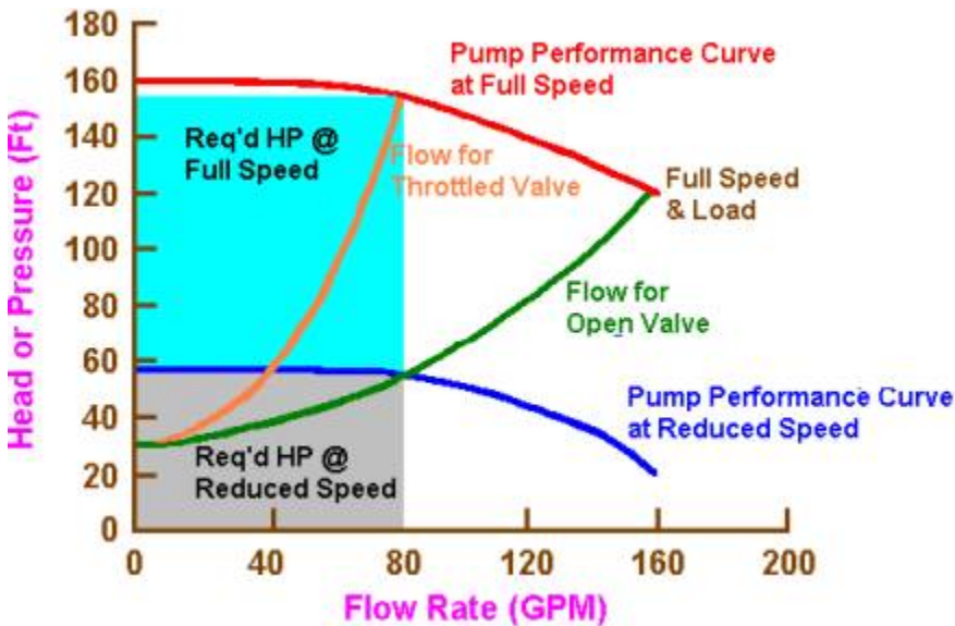
Figure 6. Speed control with throttling valve compared to variable speed control.
